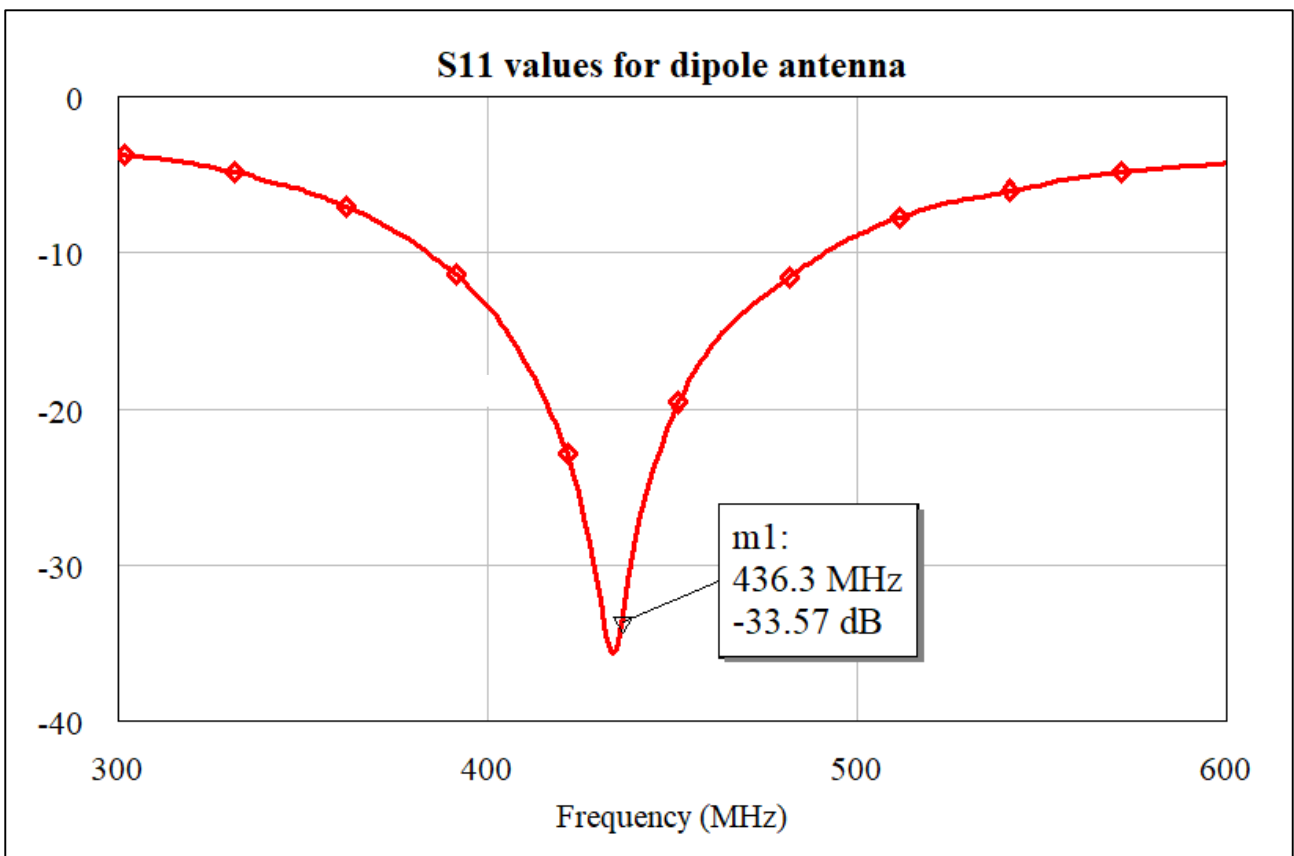
Figure2.1 S11 Variation of Frequency
