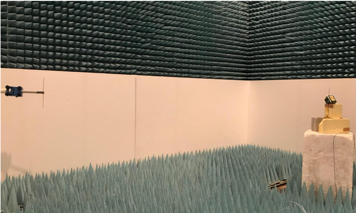
Figure1.1 Anechoic Chamber Setup
