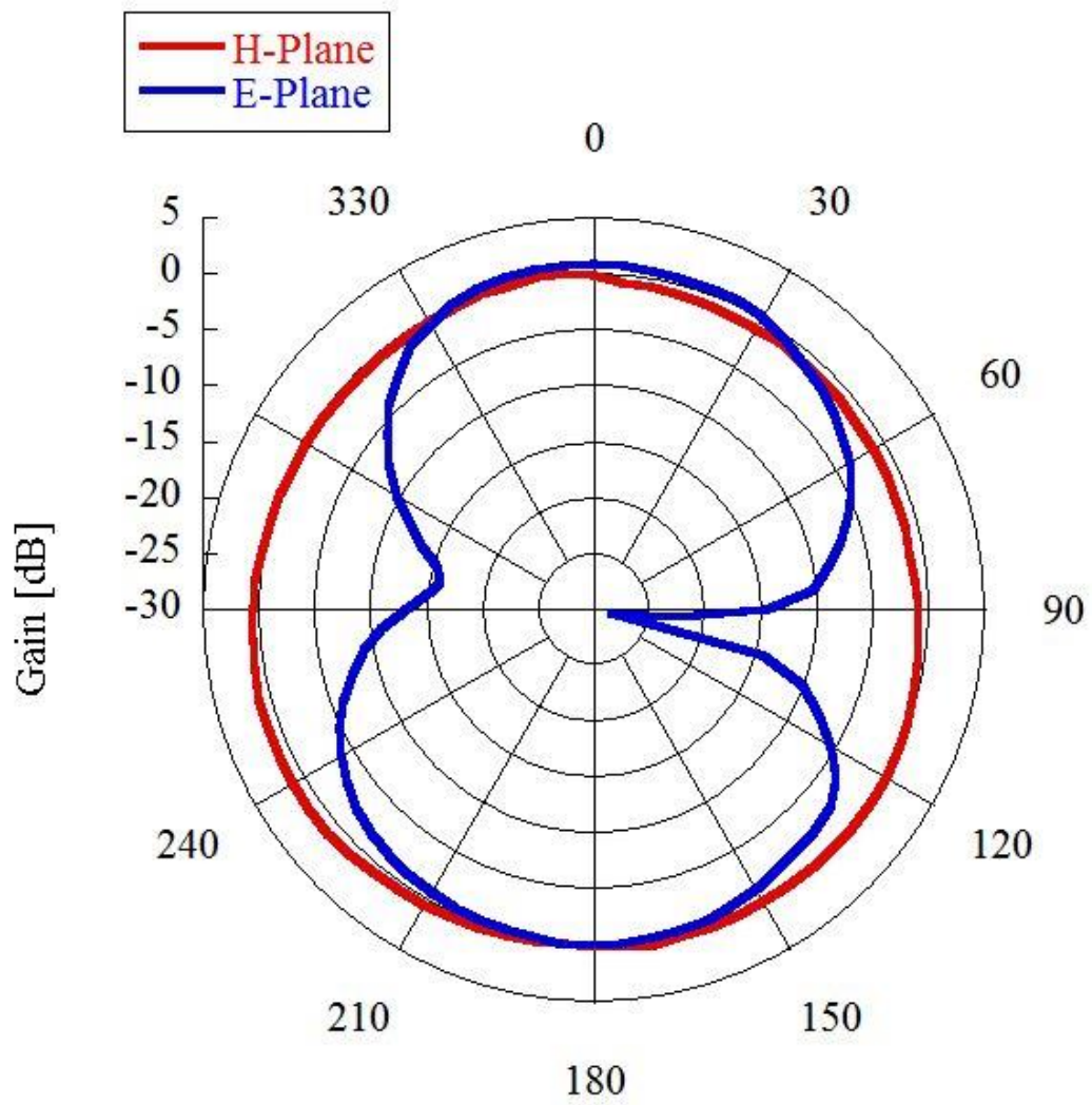
Figure 2.2 2D Antenna Radiation Pattern
